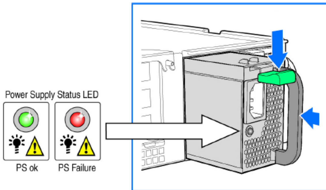
FIGURE 379 Replacing a PSU
