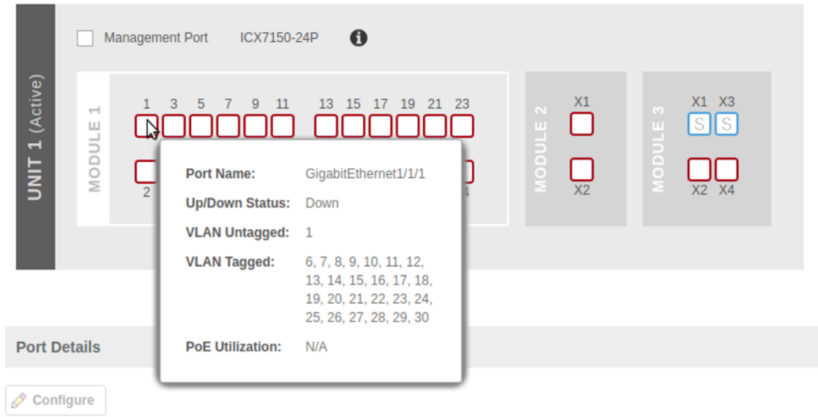
FIGURE 158 Front Panel View
